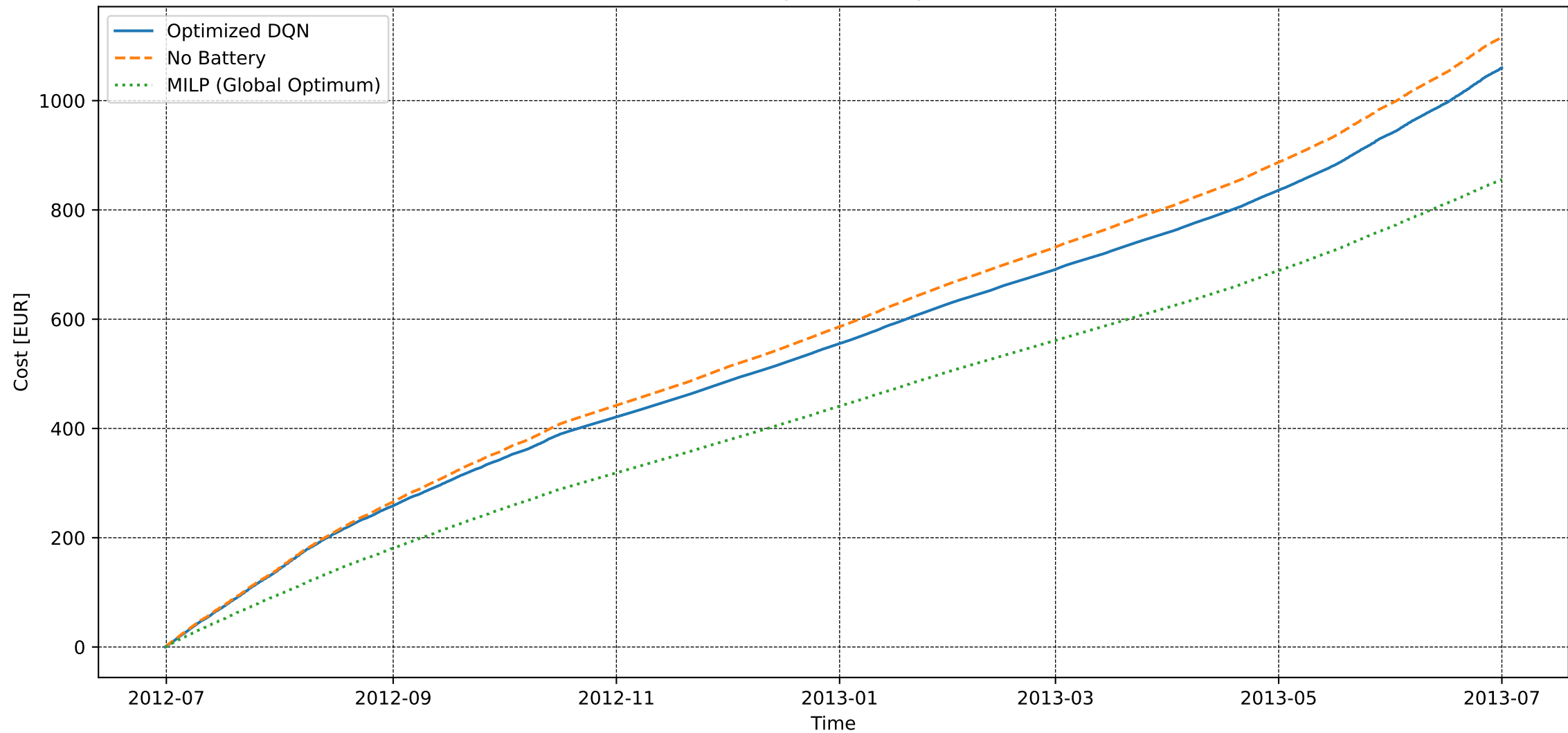
User 240 - Basic Training - Electricity Cost [DQN vs MILP]
